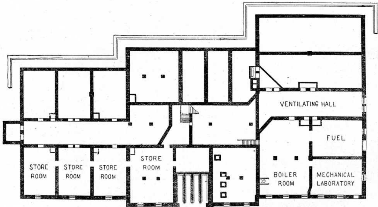
FOUNDATION PLAN.
